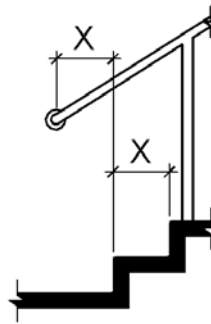
Figure 505.10.3 Bottom Handrail Extension at Stairs
