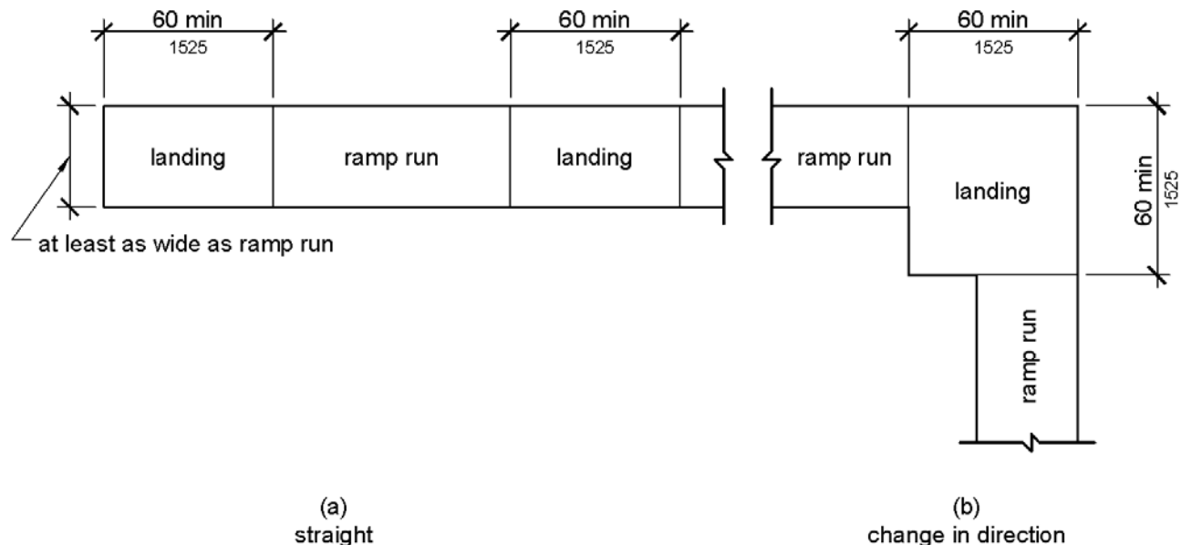
Figure 405.7 Ramp Landings
