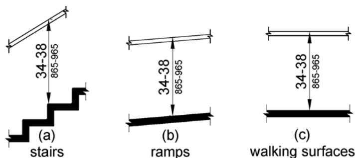
Figure 505.4 Handrail Height
